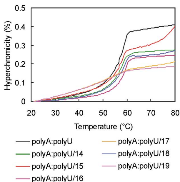
Figure 2. Thermal melting curves of polyA:polyU in the absence or presence of synthetic glycosyl nucleoside.
