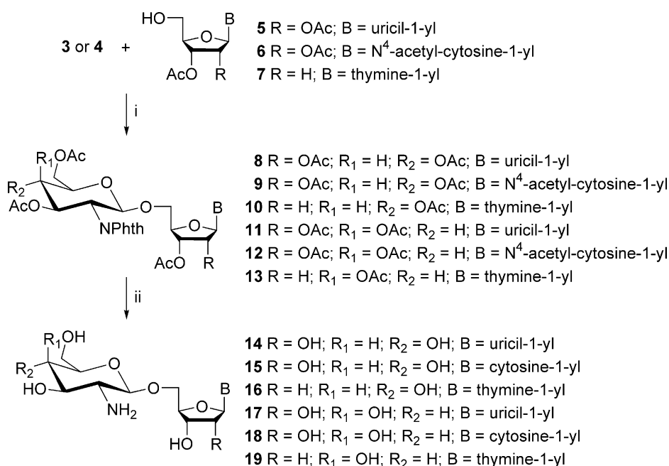
Scheme 2. Reagents and conditions: (i) BF 3 /Et 2 O, CH 2 Cl 2 , rt; (ii) (a) MeNH 2 /EtOH, rt, 8 h; (b) reflux, 6 h.
