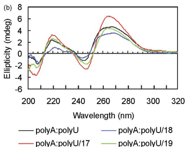
Figure 1. CD spectra of polyA:polyU in the absence or presence of synthetic glycosyl nucleoside.
