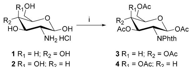
Scheme 1. Reagents and conditions: (i) (a) NaOMe, HOAc, rt, 30 min; (b) phthalic anhydride, rt, 15 h; (c) Ac 2 O, pyridine, rt, 24 h.
